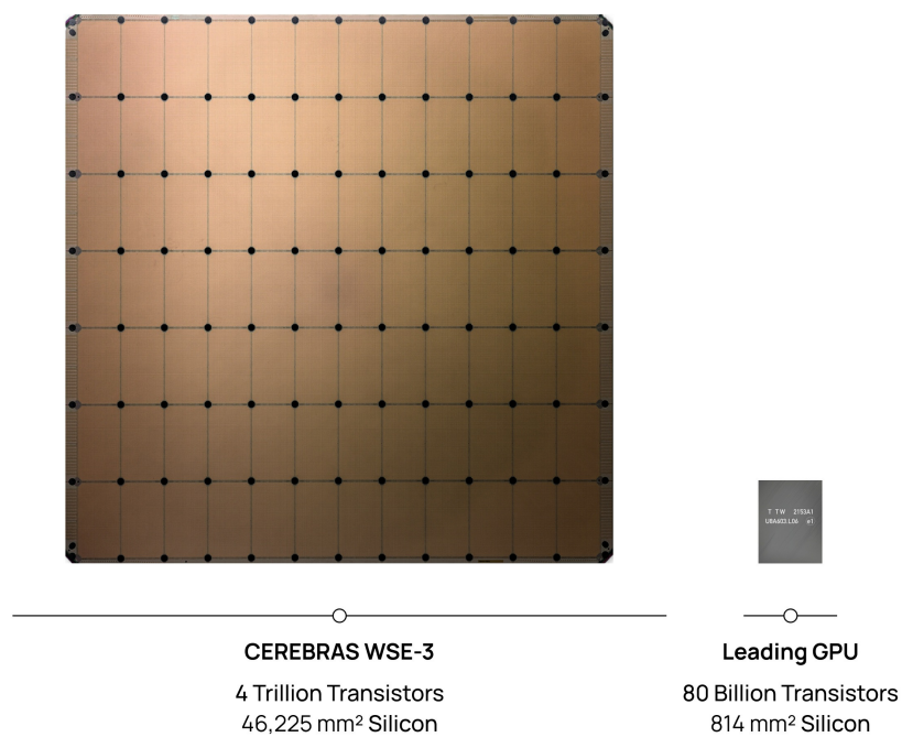
Cerebras Wafer-Scale Engine 3 Versus NVIDIA H100 Size Comparison Image is illustrative; scale is approximate.
