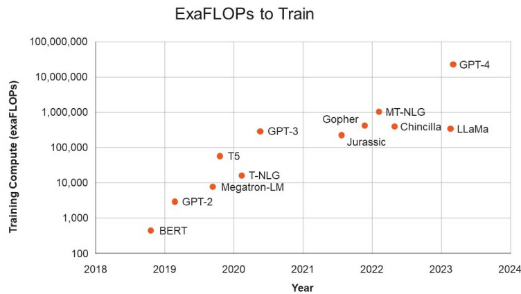
Illustration of Growing Compute Requirements Over Time (ExaFLOPS to Train LLMs)
