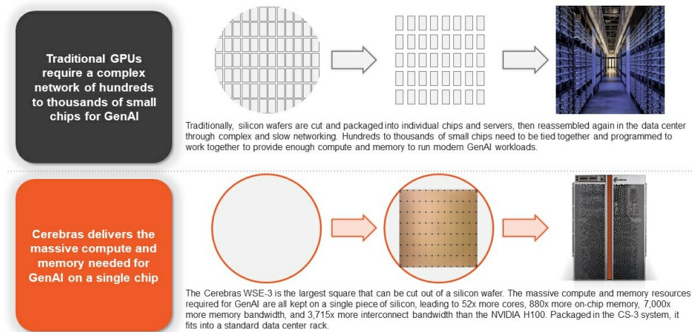
Comparison of Cerebras Wafer-Scale Integration Versus Traditional GPU Cluster Integration
