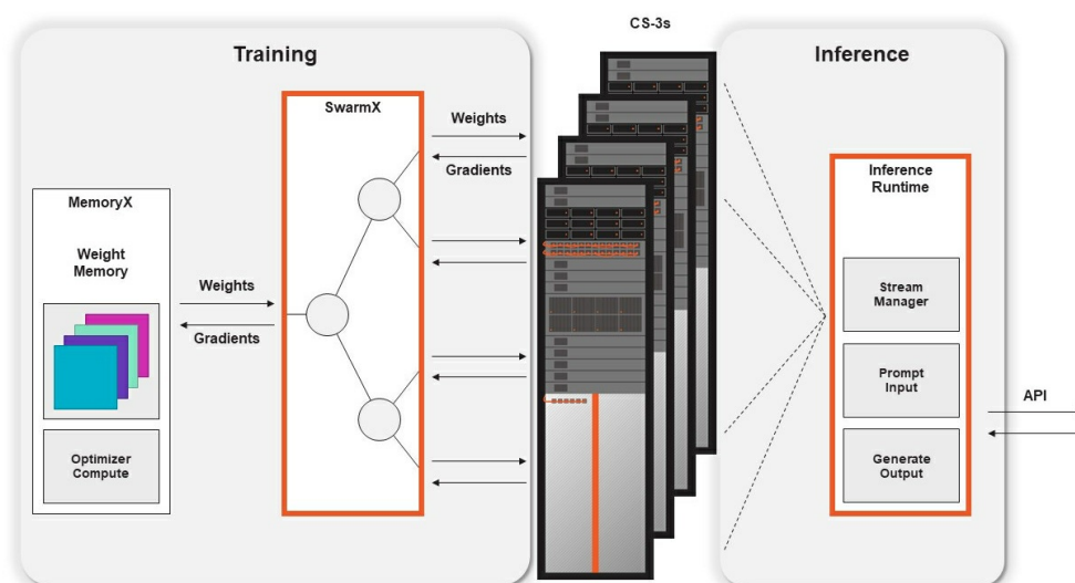
The Cerebras Wafer-Scale Cluster. The single cluster architecture has resources to support training (shown on the left) and inference (shown on the right). These resources are assigned to CS-3 systems (shown in the middle) such that any CS-3 system can be used either for training or inference.
